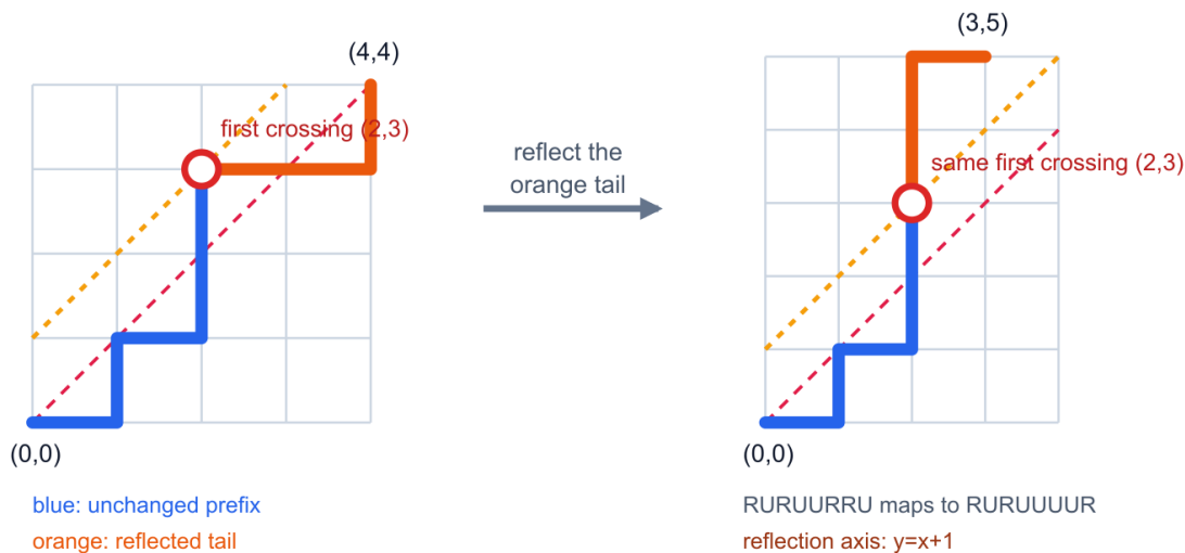
Figure 3: Reflecting the tail after the first crossing changes a bad path to (4,4) into a path to (3,5) . The construction is reversible.
