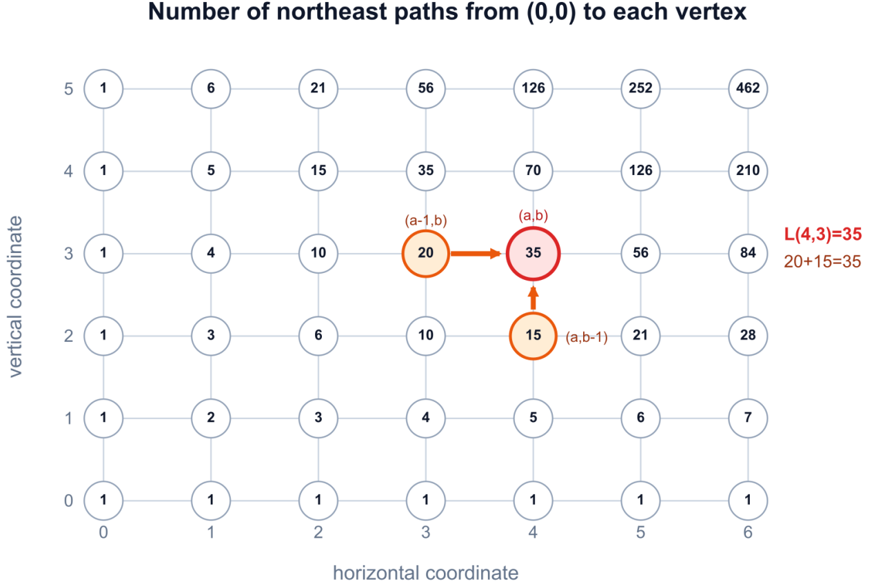
Figure 1: A recursive table of northeast-path counts. The highlighted point (a, b) = (4, 3) can be reached from (3, 3) in 20 ways and from (4, 2) in 15 ways, so its label is 20 + 15 = 35 .
