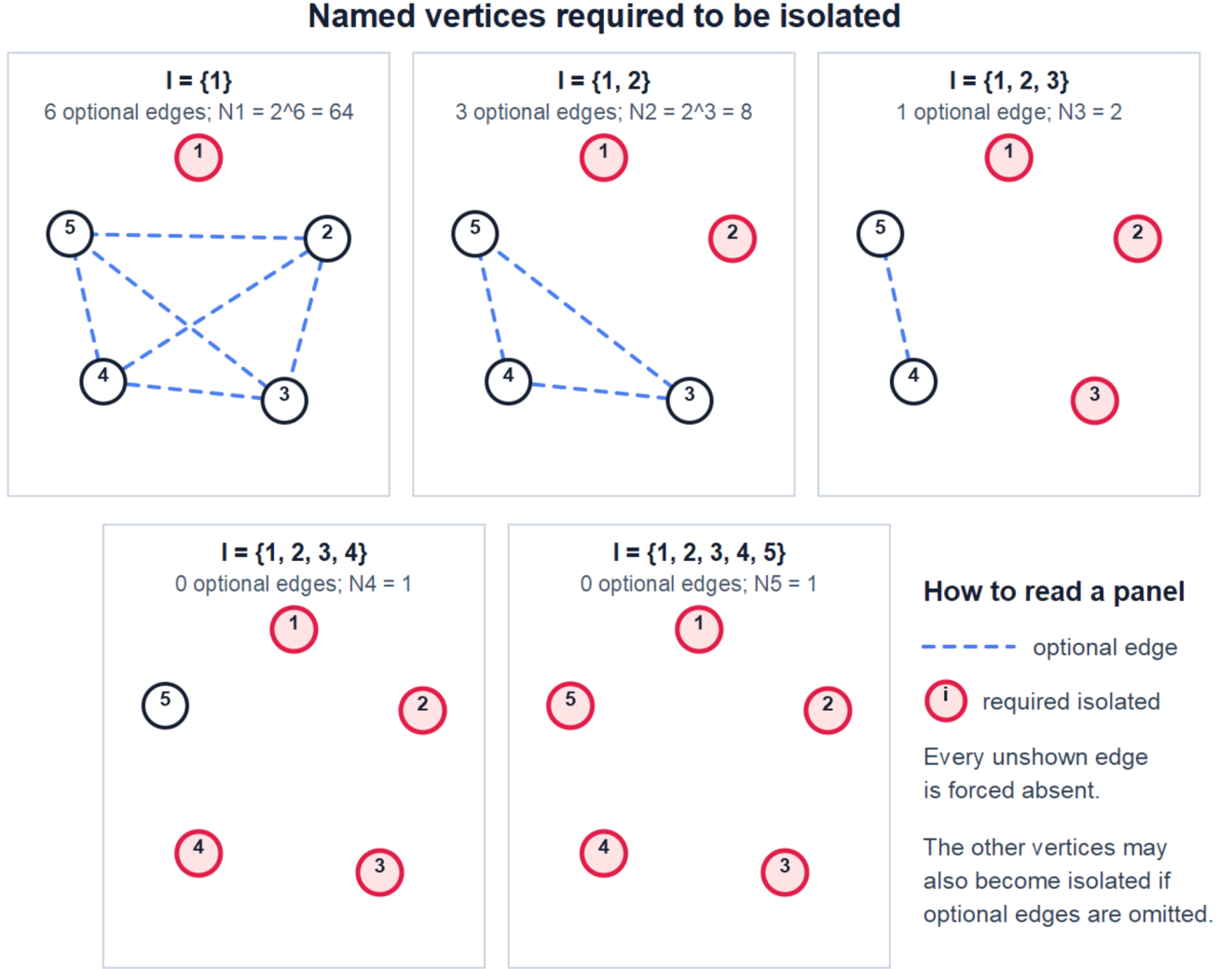
Figure 4: Representative intersections of k isolated-vertex conditions for graphs on [5] . After those conditions are imposed, only edges among the other 5 - k vertices remain optional.
