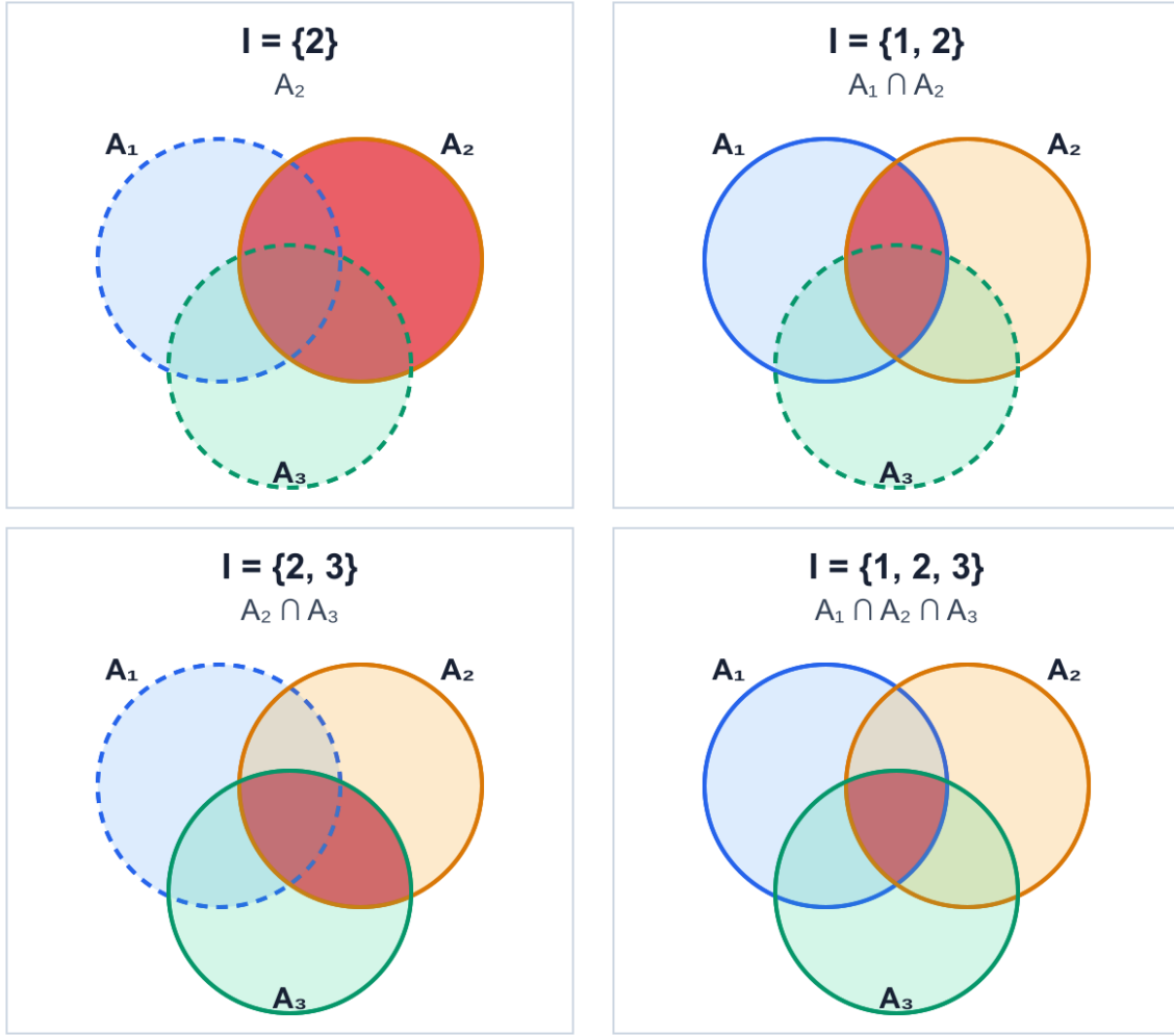
Figure 2: Four intersections corresponding to index subsets of \{1, 2, 3\} : I = \{2\} gives A_2 ; I = \{1, 2\} gives A_1 \cap A_2 ; I = \{2, 3\} gives A_2 \cap A_3 ; and I = \{1, 2, 3\} gives A_1 \cap A_2 \cap A_3 .
