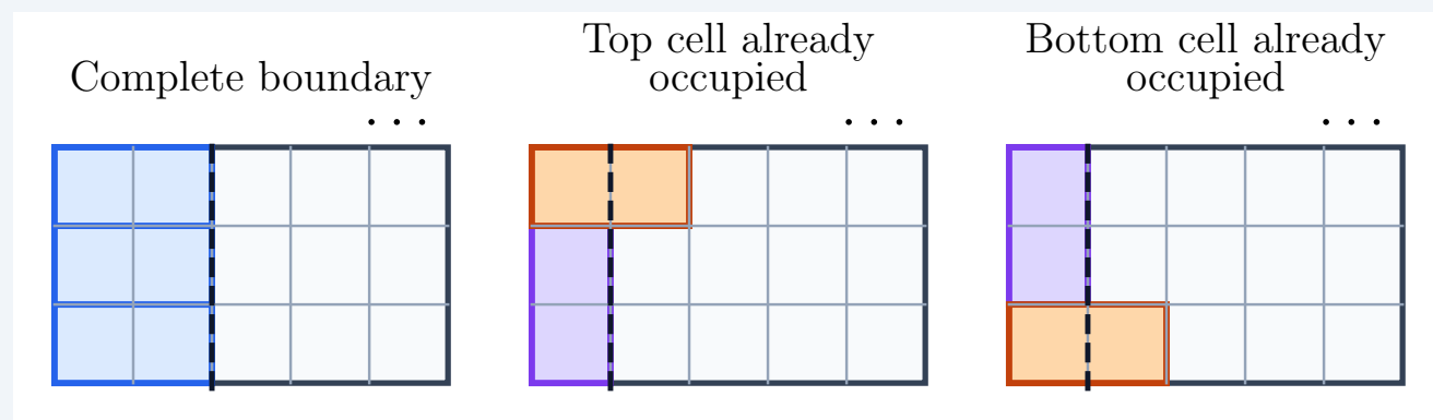
Figure 3: A cut through a 3 \times n tiling need not leave a smaller rectangle. A horizontal domino crossing the cut can leave the top or bottom square of the next column already occupied.
