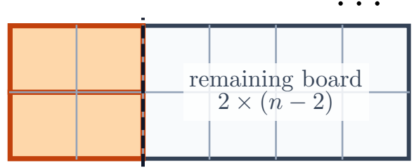
Case 2: two horizontal dominoes
