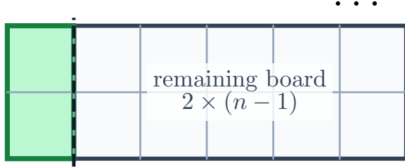
Case 1: one vertical domino
