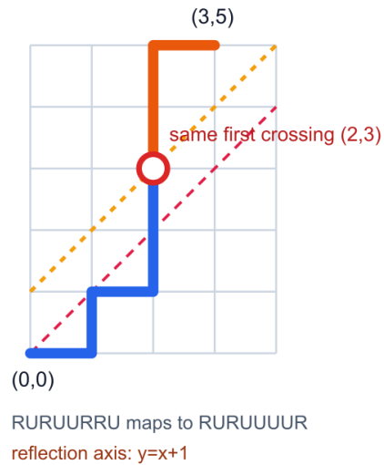
Figure 3: Reflecting the tail after the first crossing changes a bad path to (4,4) into a path to (3,5) . The construction is reversible.
