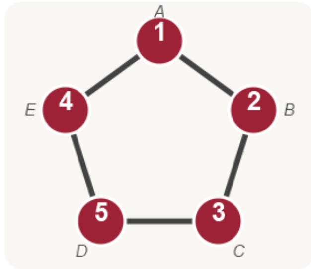
Figure 3: A nonrotation of Pattern 1 using digits 1, 2, 3, 5, 4. Figure description: Pentagon with digits 1, 2, 3, 5, 4 clockwise from the top vertex.
