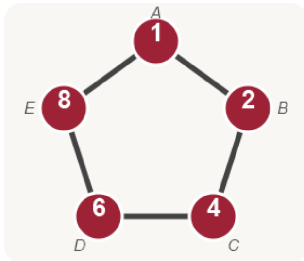
Figure 4: A pattern using digits 1, 2, 4, 6, 8. Figure description: Pentagon with digits 1, 2, 4, 6, 8 clockwise from the top vertex.
