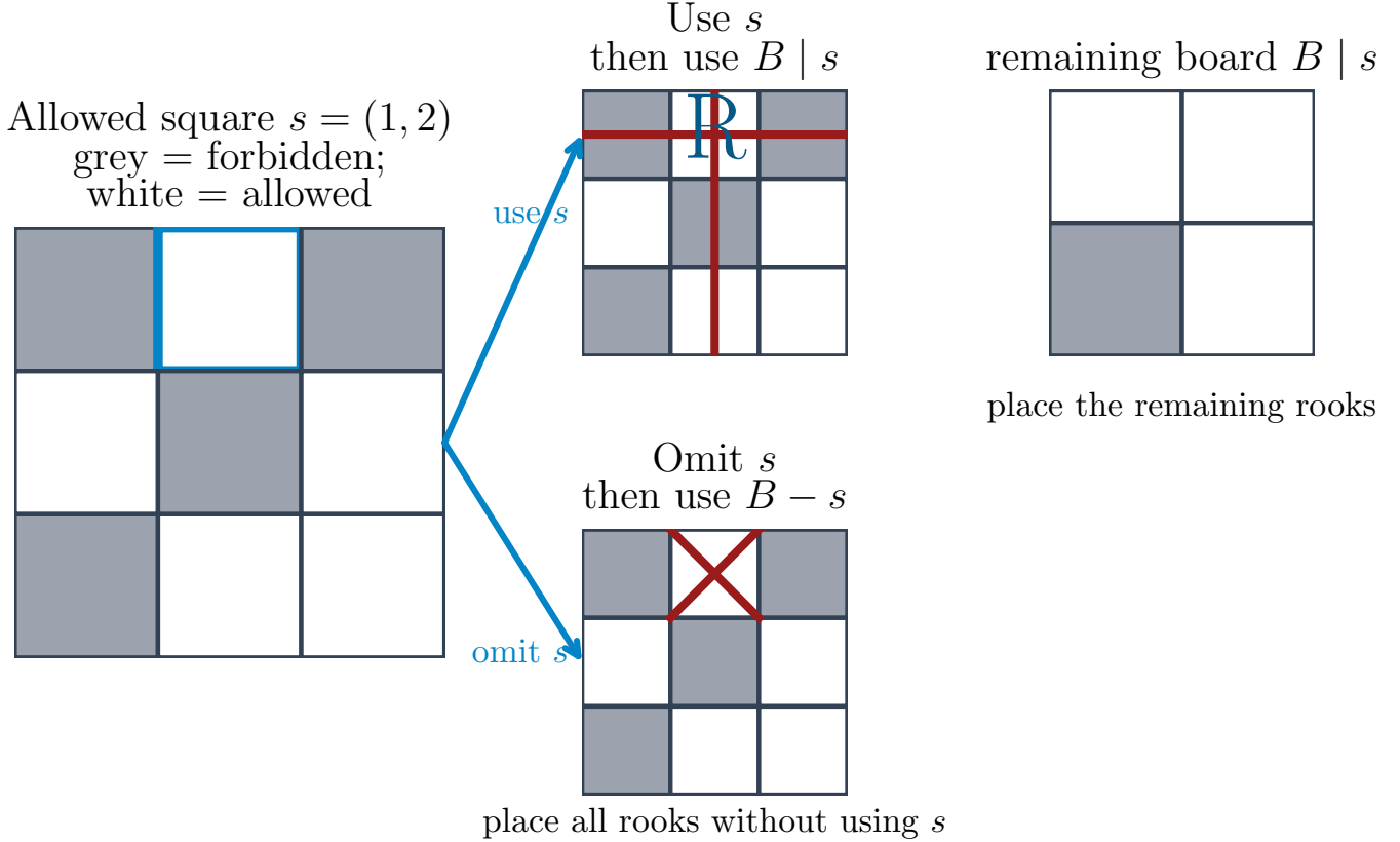
Figure 6: The two classes of legal rook placements at the white allowed square s = (1,2) . Using s fixes one legal assignment and leaves the smaller allowed board B \mid s . Omitting s leaves the allowed board B - s .
