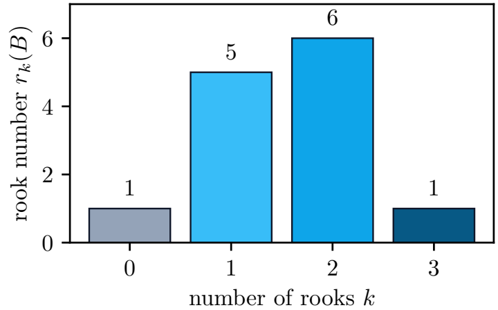
Figure 4: A direct count of the rook numbers for B . The five allowed cells give r_1(B) = 5 ; six unordered pairs use different rows and columns; exactly one three-rook placement is possible; and these values become the coefficients of R_B(x) .
