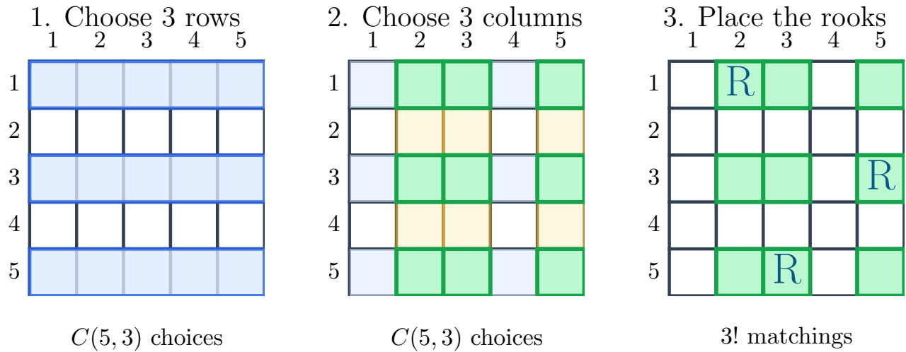
Figure 2: Counting three nonattacking rooks on a full five-by-five board. Select three rows, select three columns, and then choose a bijection between the selected rows and columns.
