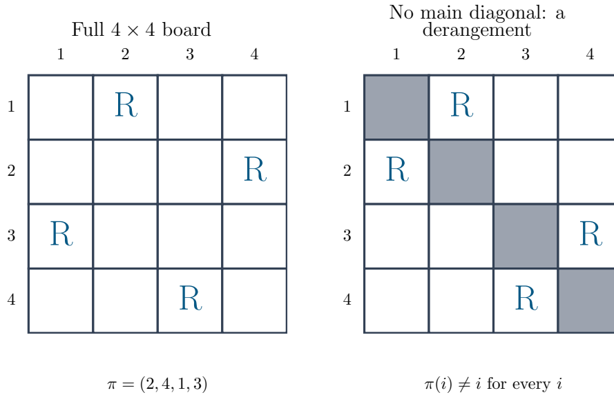
Figure 1: A full four-by-four board and the board obtained by removing its main diagonal. A full placement represents a permutation; a full placement avoiding the grey diagonal squares represents a derangement.
