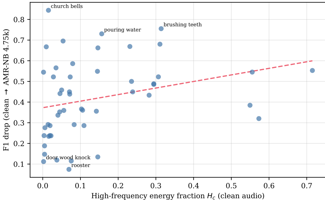
Per-class vulnerability vs high-frequency reliance ESC-50, n = 50 classes ( \rho = 0.40 , p = 0.004 )
