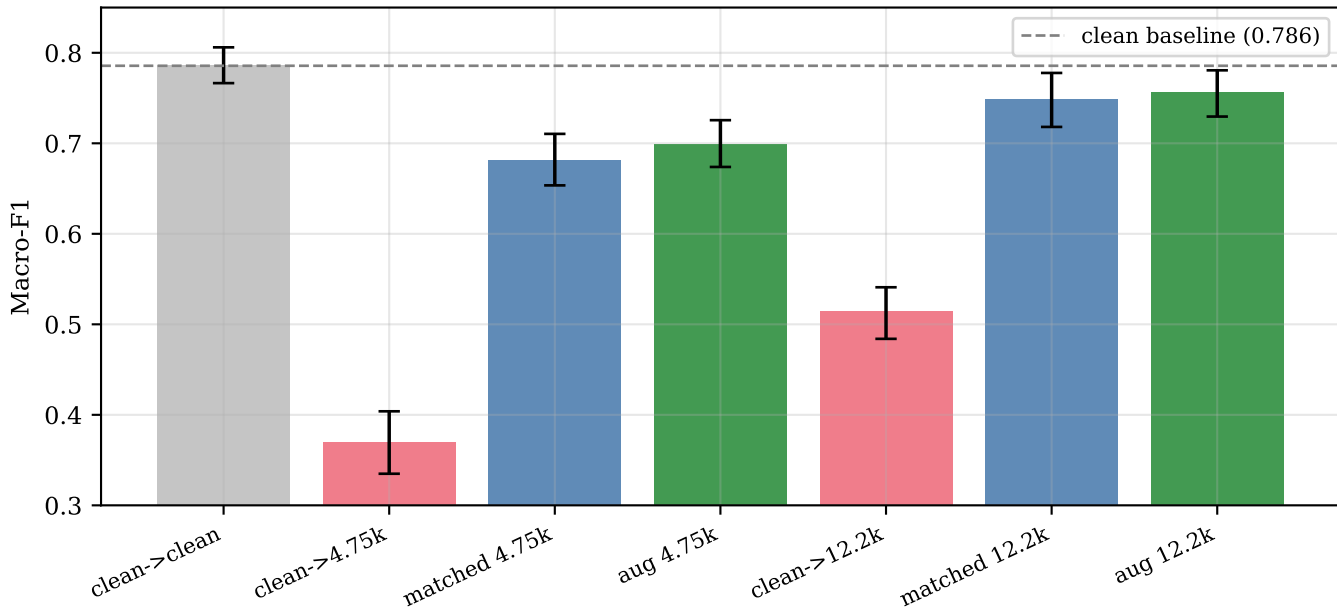
Training regime comparison with 95% CI (ResNet-50)
