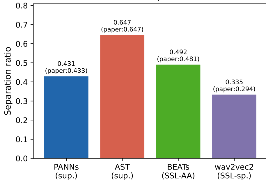
(a) Class separation
