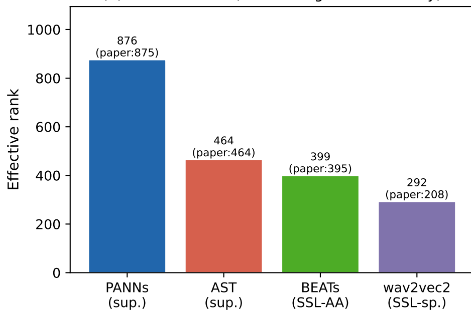
(b) Effective rank (embedding dimensionality)
