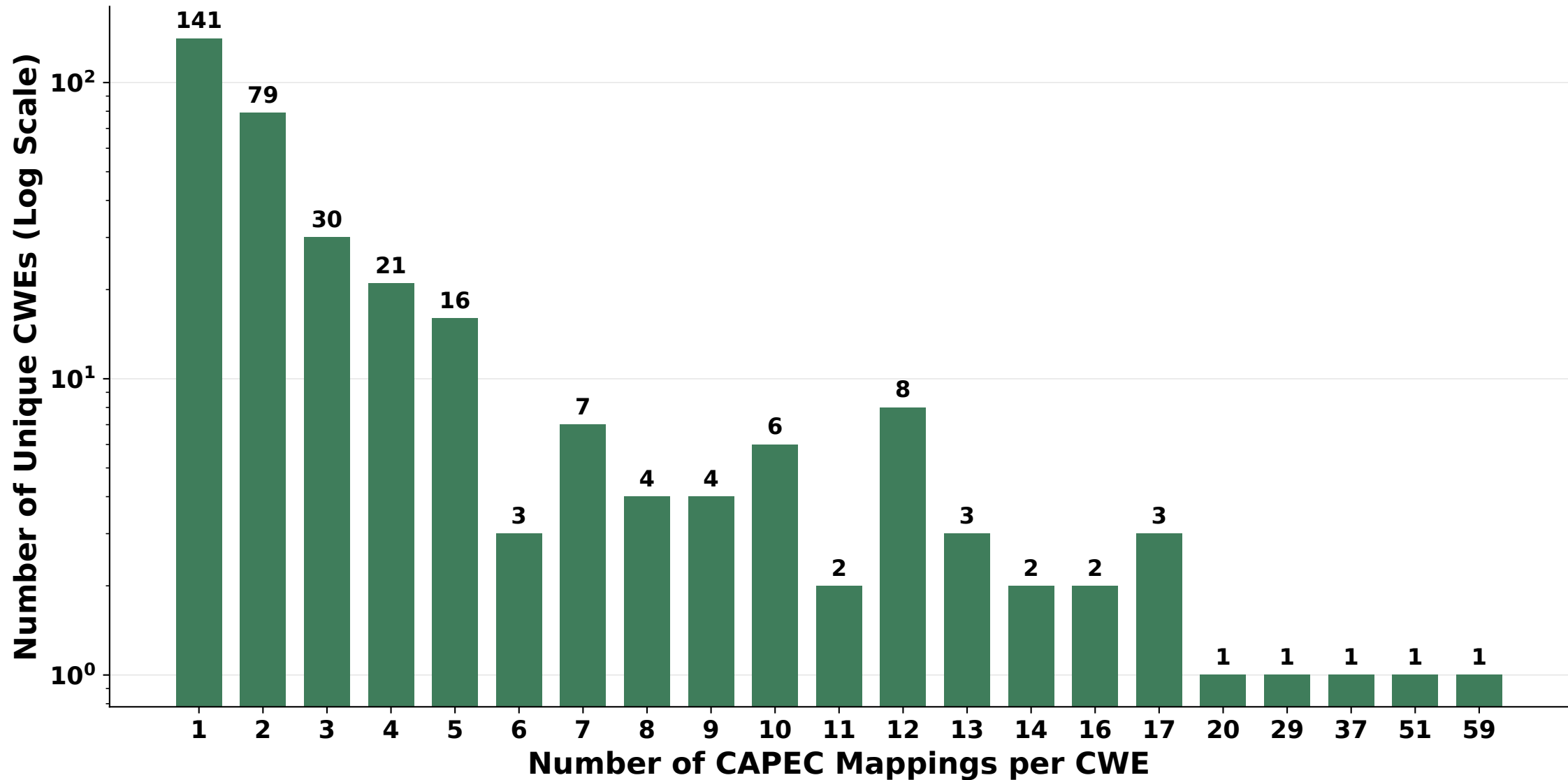
Distribution of CAPEC Mappings Across CWE
