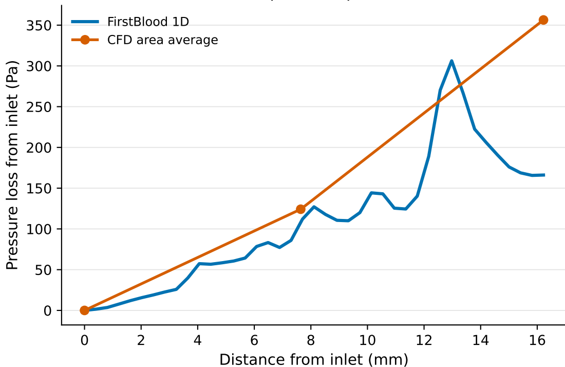
TM2 pressure profile
