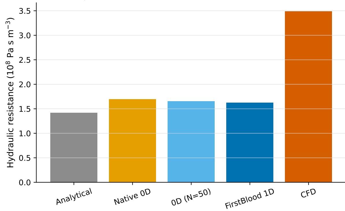
Hydraulic resistance on the common CFD domain
