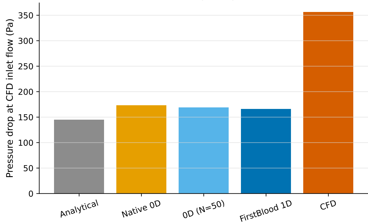
Pressure-drop comparison
