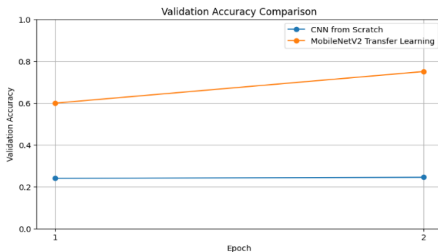
Figure 4: Comparison of validation accuracy between the CNN trained from inception and the MobileNetV2 transfer learning model.
