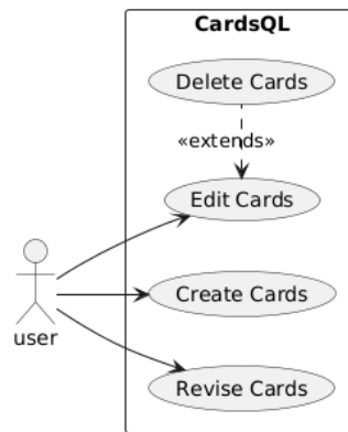
Figure 3.1: Use case diagram for CardsQL
