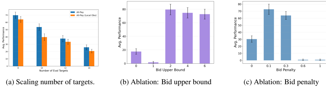
Figure 5: Scaling number of targets and ablations on the Cat Feeder environment.
