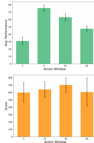
Figure 6: Effect of action window on performance: Cat Feeder (top) and Atari Assault (bottom).
