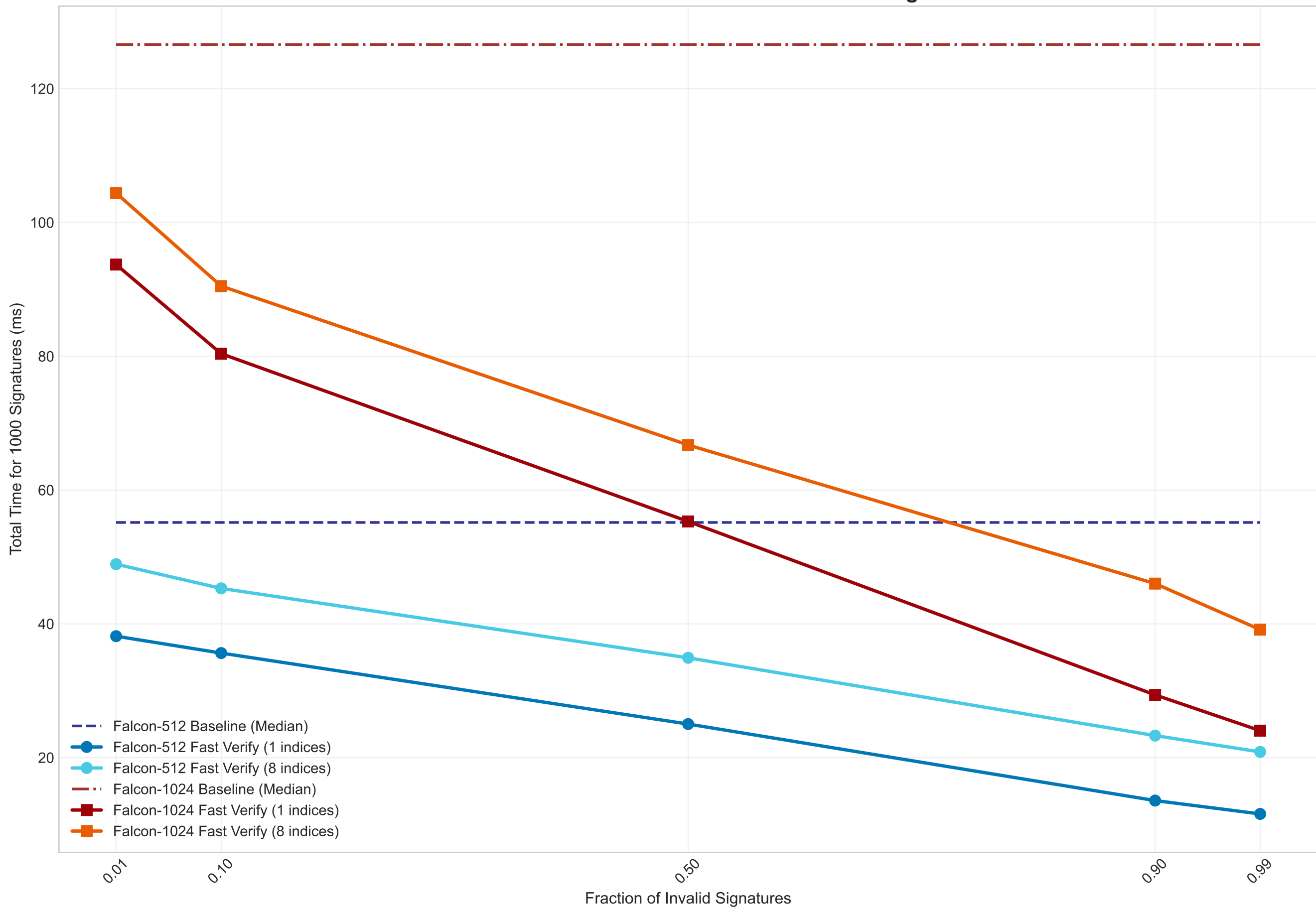
Falcon Stream Verification Benchmark: Processing Time
