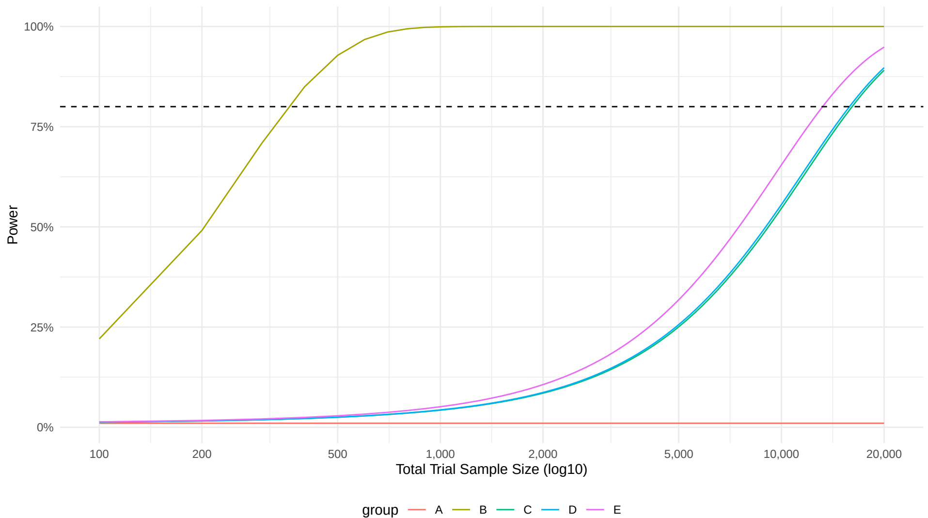
Aim 1: Power vs Sample Size (log scale)
