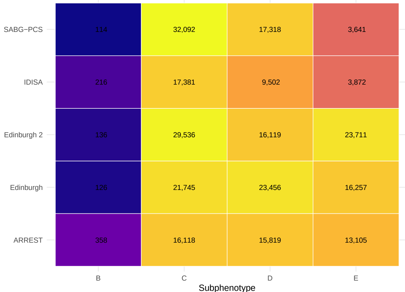
Aim 1 Sensitivity: Required N for 80% Power
