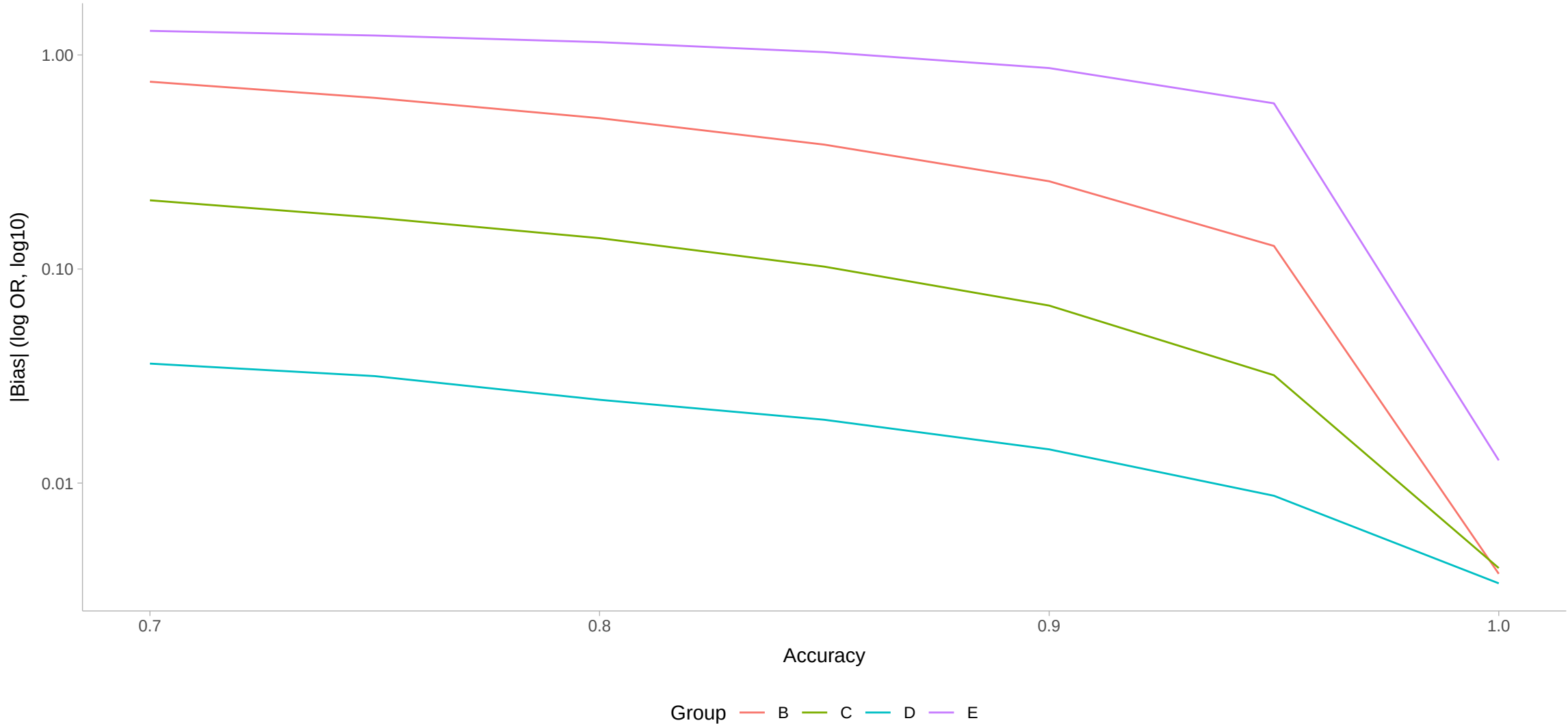
Aim 2: |Bias| vs Accuracy (log y)
