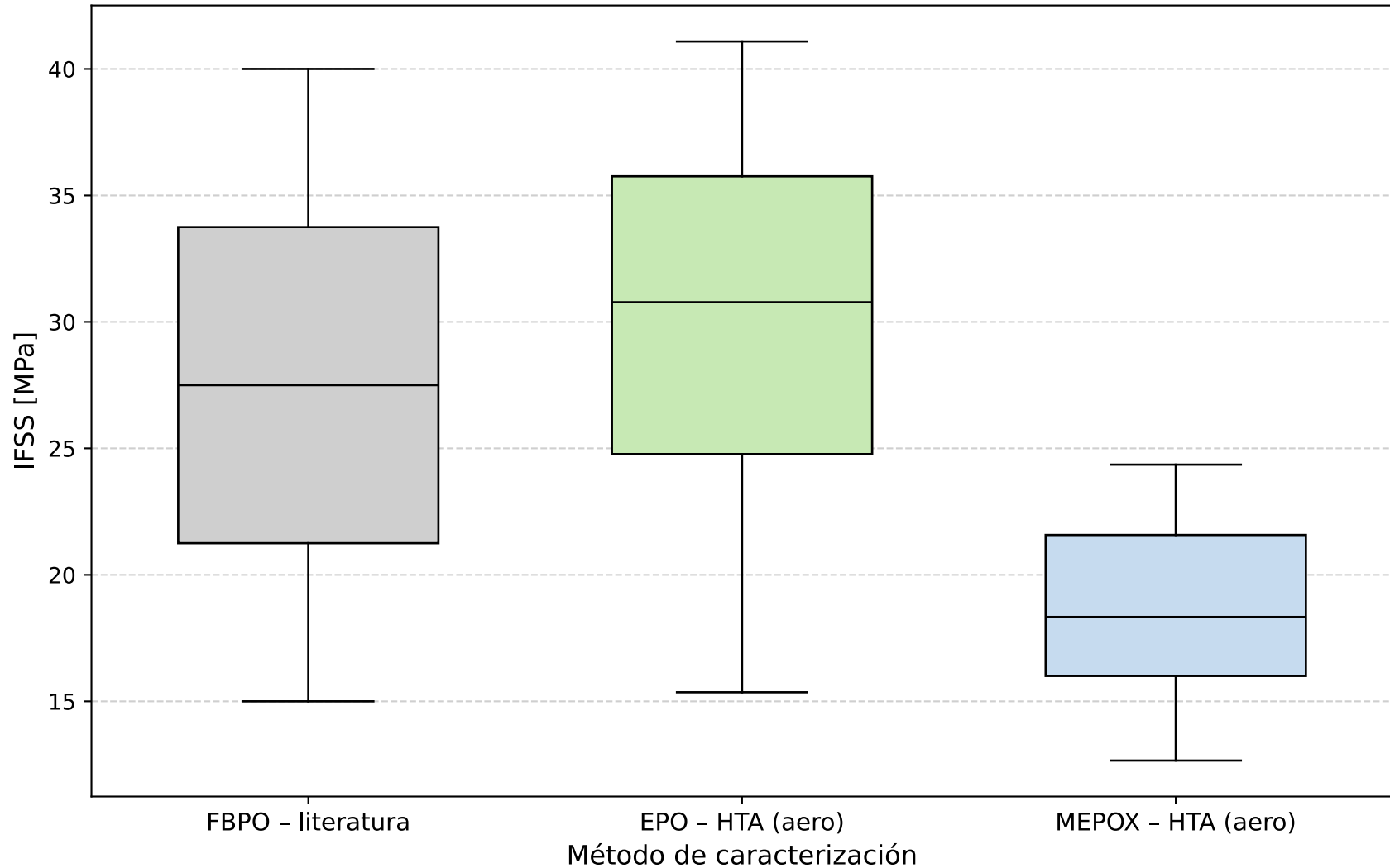
Comparativa IFSS: literatura vs experimental
