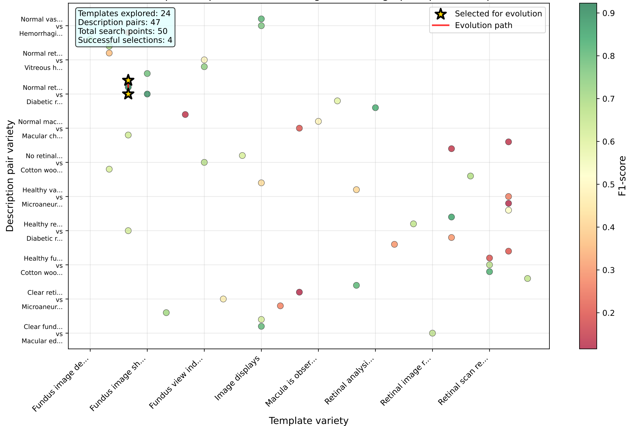
Search space exploration: APE navigation through prompt landscape
