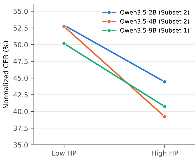
(b) Out-of-distribution
