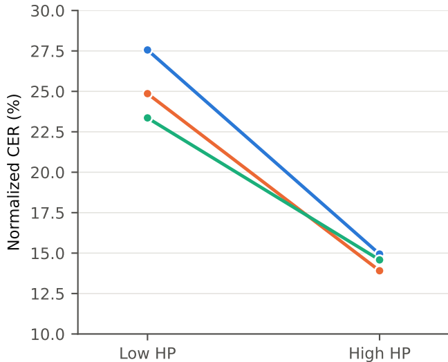
(a) In-distribution
