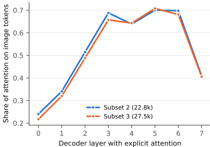
(a) Mean share per layer
