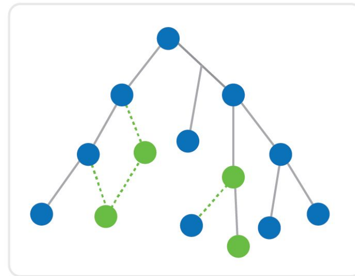
Accessibility Tree
