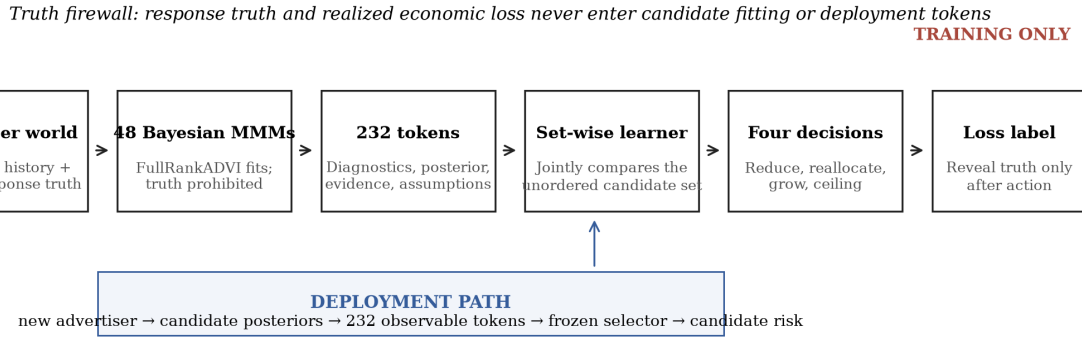
Figure 1. Research and deployment paths. Hidden causal truth is opened only after a candidate has acted in simulation. Deployment uses the frozen mapping from observable candidate sets to predicted decision risk.
