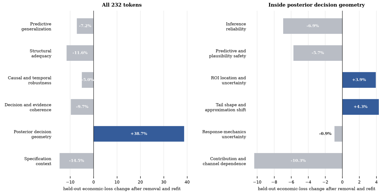
Figure 8. Advertiser-grouped development importance. Bars show the percentage change in held-out economic loss when a complete token group is removed and the selector is relearned. Positive values indicate incremental predictive information; gray negative values indicate conditional redundancy or finite-sample overfit, not that the underlying scientific check is unnecessary. The sealed cohort was not opened for this analysis.
