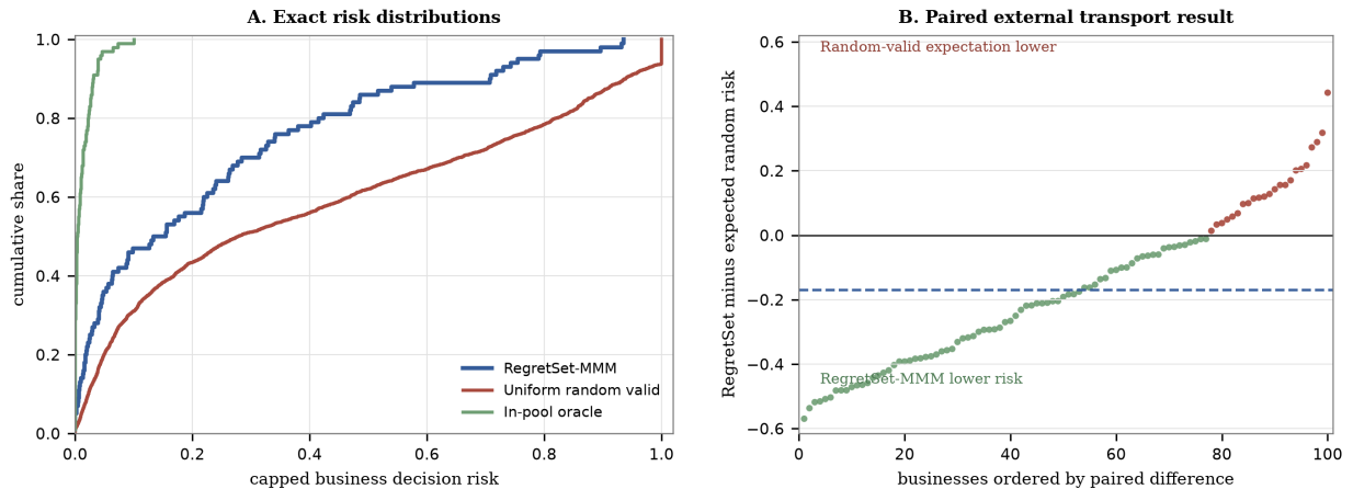
Figure 7. External AMSS transport. Panel A shows the exact capped-risk distributions for the frozen RegretSet-MMM selector, uniform random selection among valid candidates, and the truth-informed in-pool oracle. Panel B shows paired RegretSet-MMM risk minus each business's expected random-valid risk; values below zero favor RegretSet-MMM.
