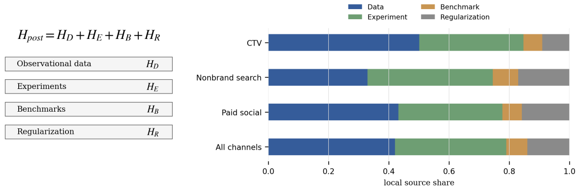
Figure 4. Observed local evidence attribution for the 1,260 channel posteriors in the 420 outer-fold selected development candidates. Bars report equal-channel mean Laplace curvature shares. Overall, observational data supplied 42.1%, experiments 36.9%, benchmarks 7.0%, and regularization 14.0% of local ROI information. These are development-cohort influence estimates, not scores of source validity.
