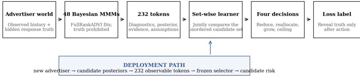
Figure 1. Research and deployment paths. Hidden causal truth is opened only after a candidate has acted in simulation. Deployment uses the frozen mapping from observable candidate sets to predicted decision risk.
