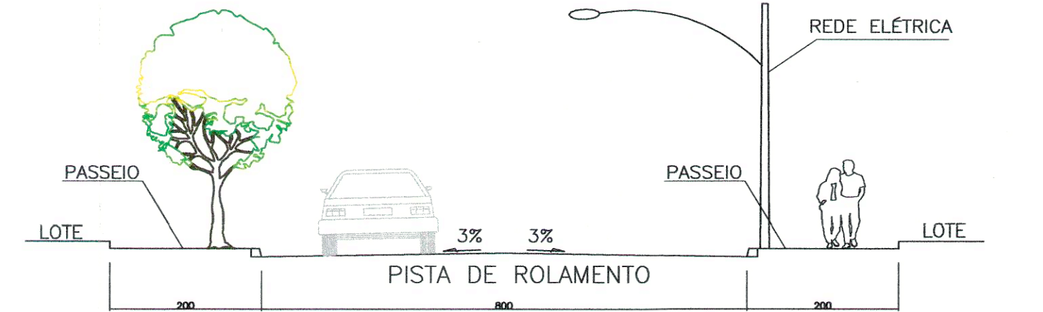
SEÇÃO TRANSVERSAL - RUAS 12.00m RUA JL 2, JL 3, JL 4, JL 5, JL 6, JL 7 JL 8, JL 9, JL 10, JL 11, JL 12, JL 13, JL 16
