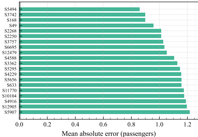
Top-20 lowest MAE stops
