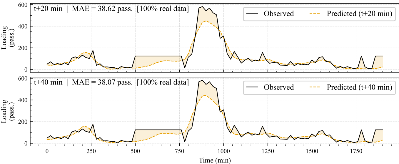
Stop 43768720 | Route 137 | Inbound (node idx: 2475) -- all forecast horizons [AGCRN]
