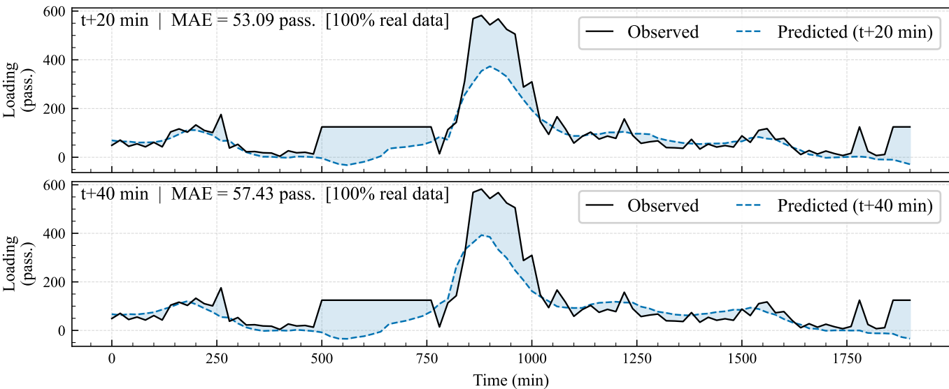
Stop 43768720 | Route 137 | Inbound (node idx: 2475) -- all forecast horizons [Graph Wavenet]
