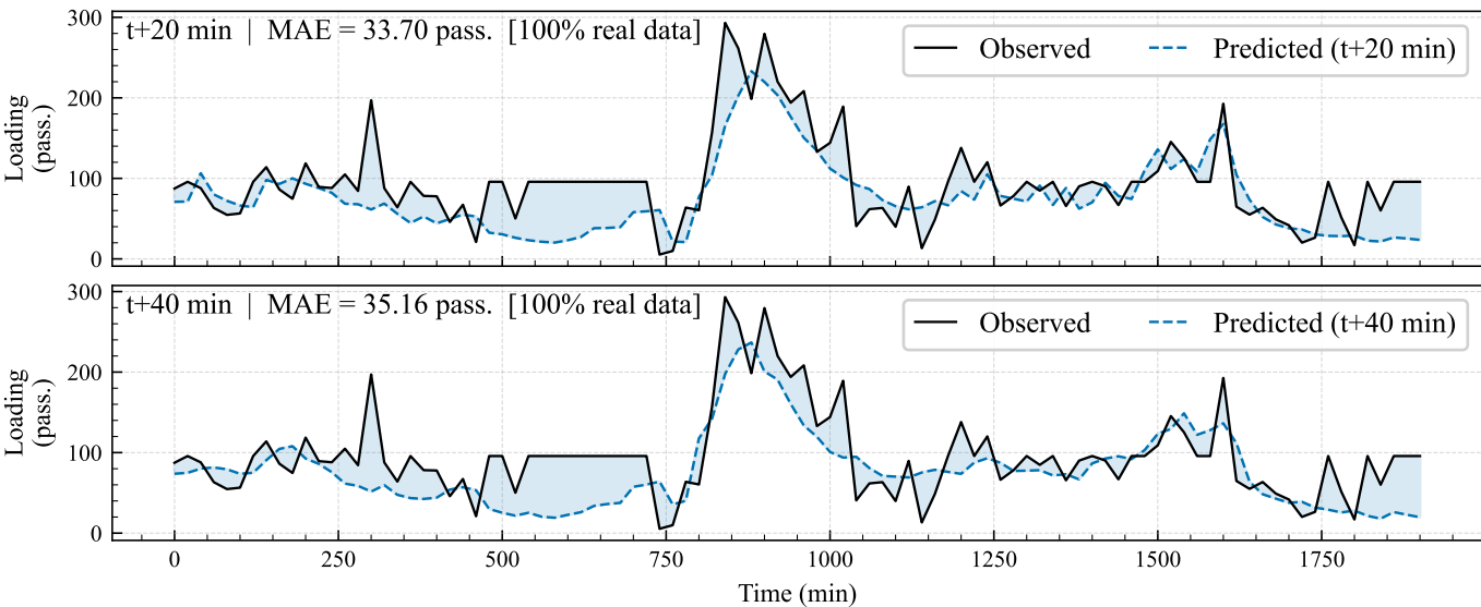
Stop 44165280 | Route 1320 | Inbound (node idx: 3496) -- all forecast horizons [Graph Wavenet]
