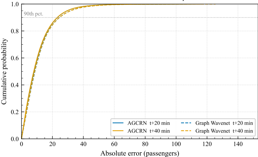
CDF of absolute error — AGCRN vs. Graph WaveNet
