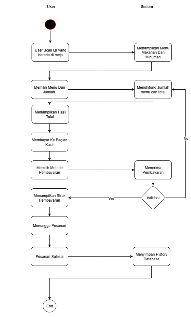
Gambar 3. 6 Activity Diagram
