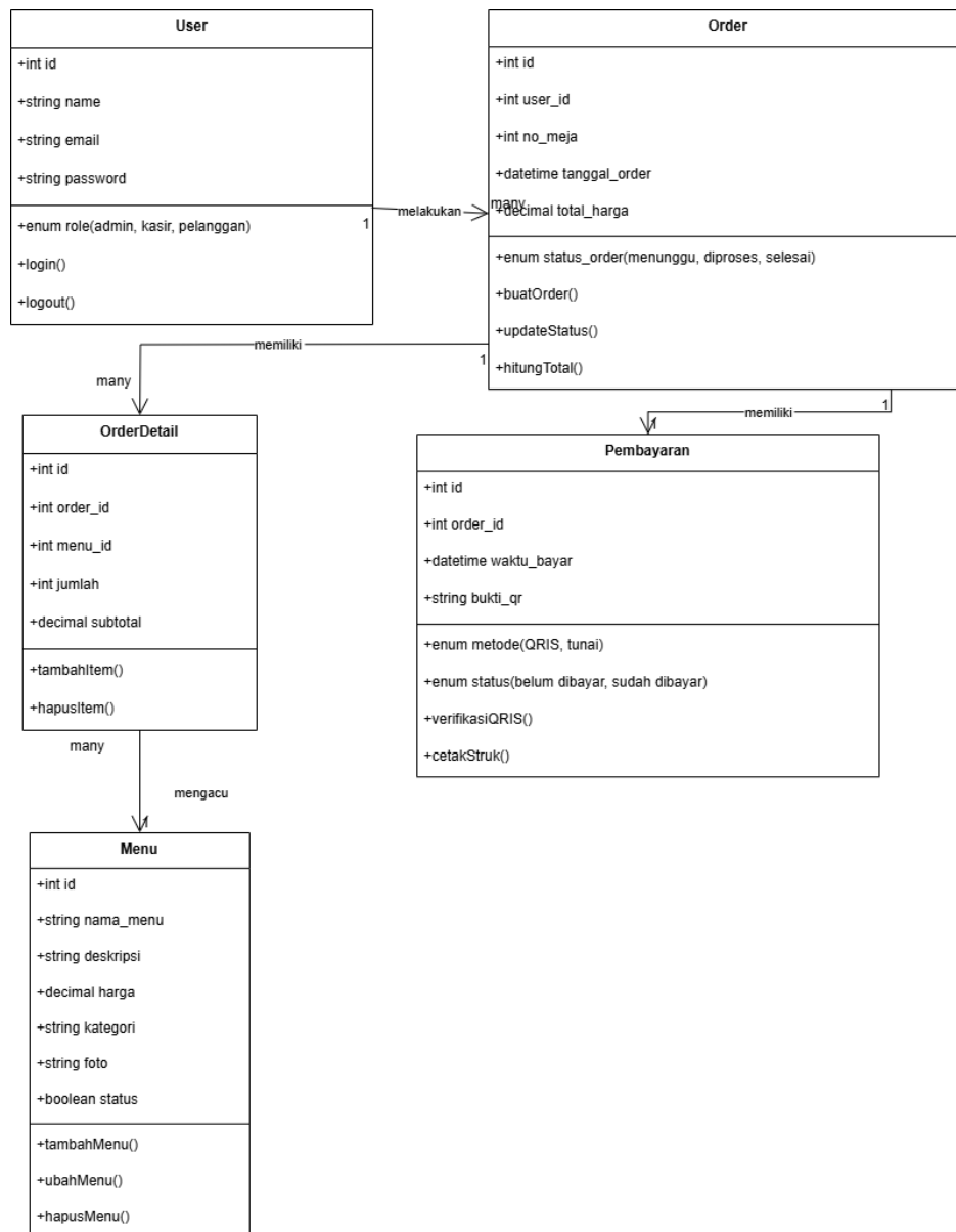
Gambar 4. 2 Class Diagram
