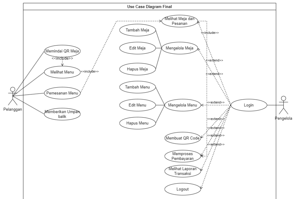
Gambar 4.1 Use Case Diagram Final (Lampiran 1)
