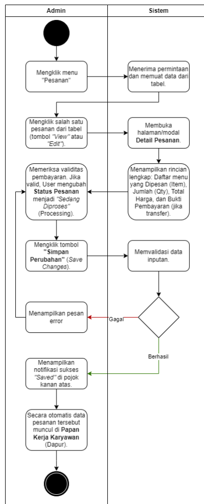
Gambar 4.7 Activity Diagram Pesanan (Lampiran 7)
