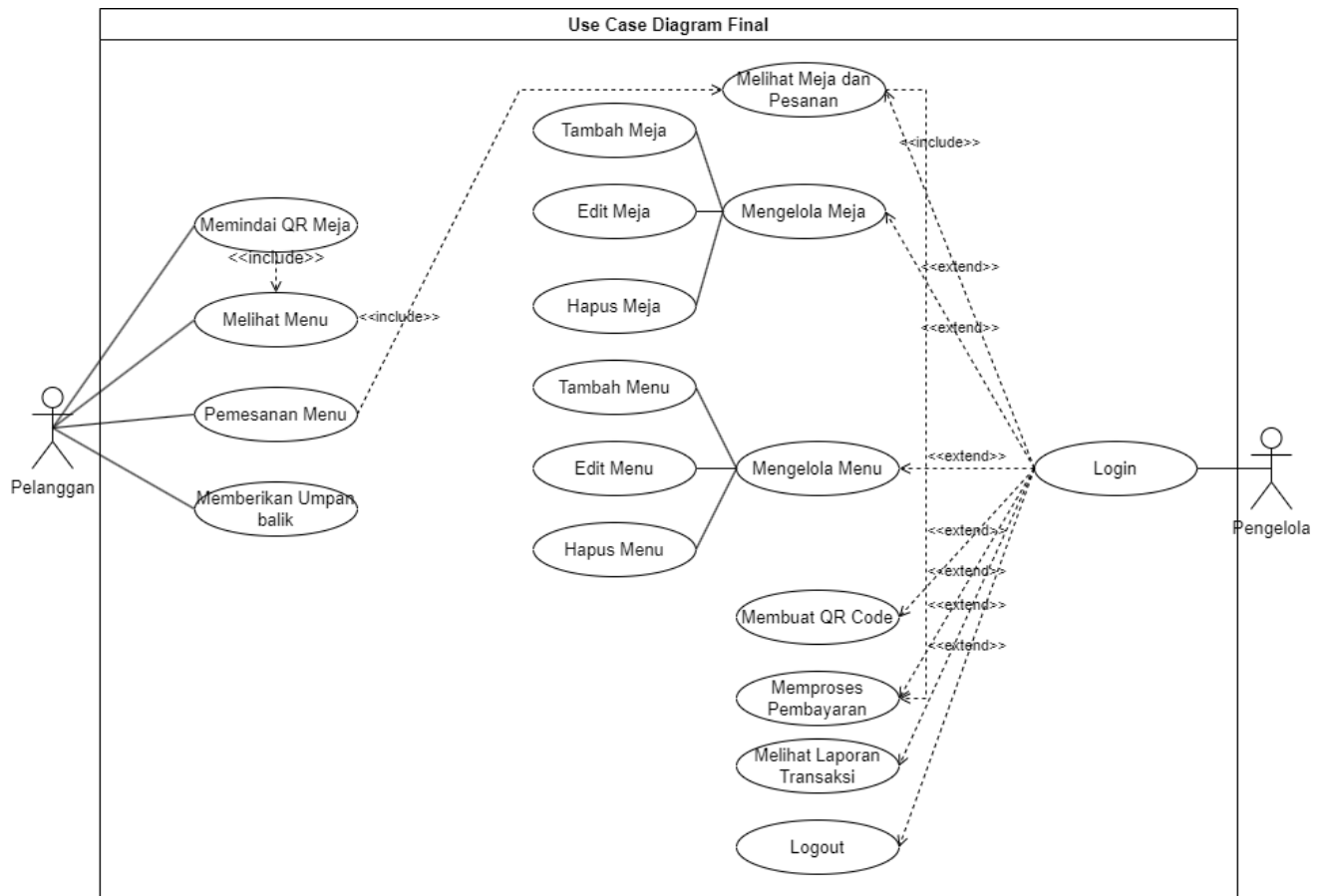
Lampiran 1 Use Case Diagram Final
