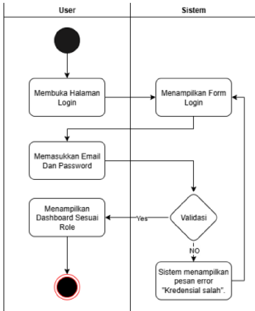
Gambar 4.3 Activity Diagram Login
