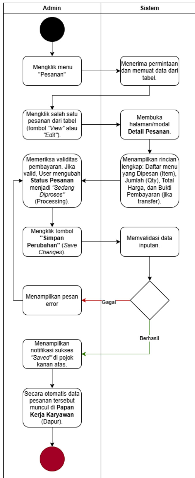
Lampiran 7 Activity Diagram Pesanan
