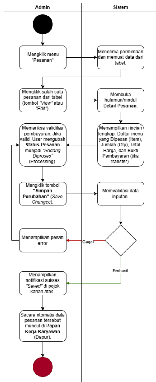
Gambar 4. 7 Activity Diagram Pesanan
