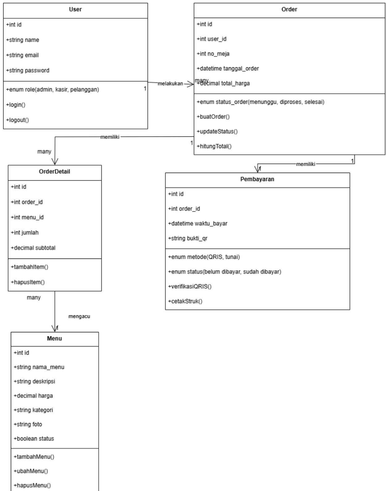
Gambar 3.5 Class Diagram
