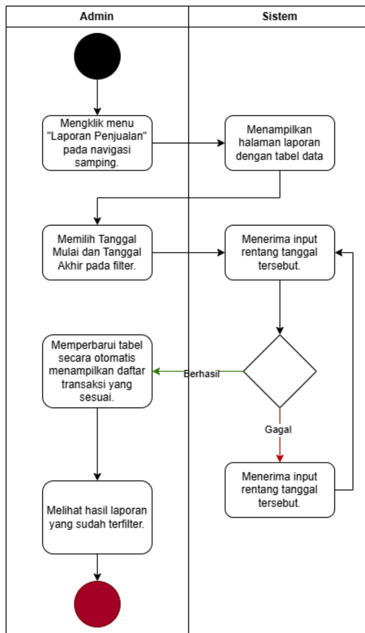
Gambar 4. 10 Activity Diagram Laporan Penjualan
