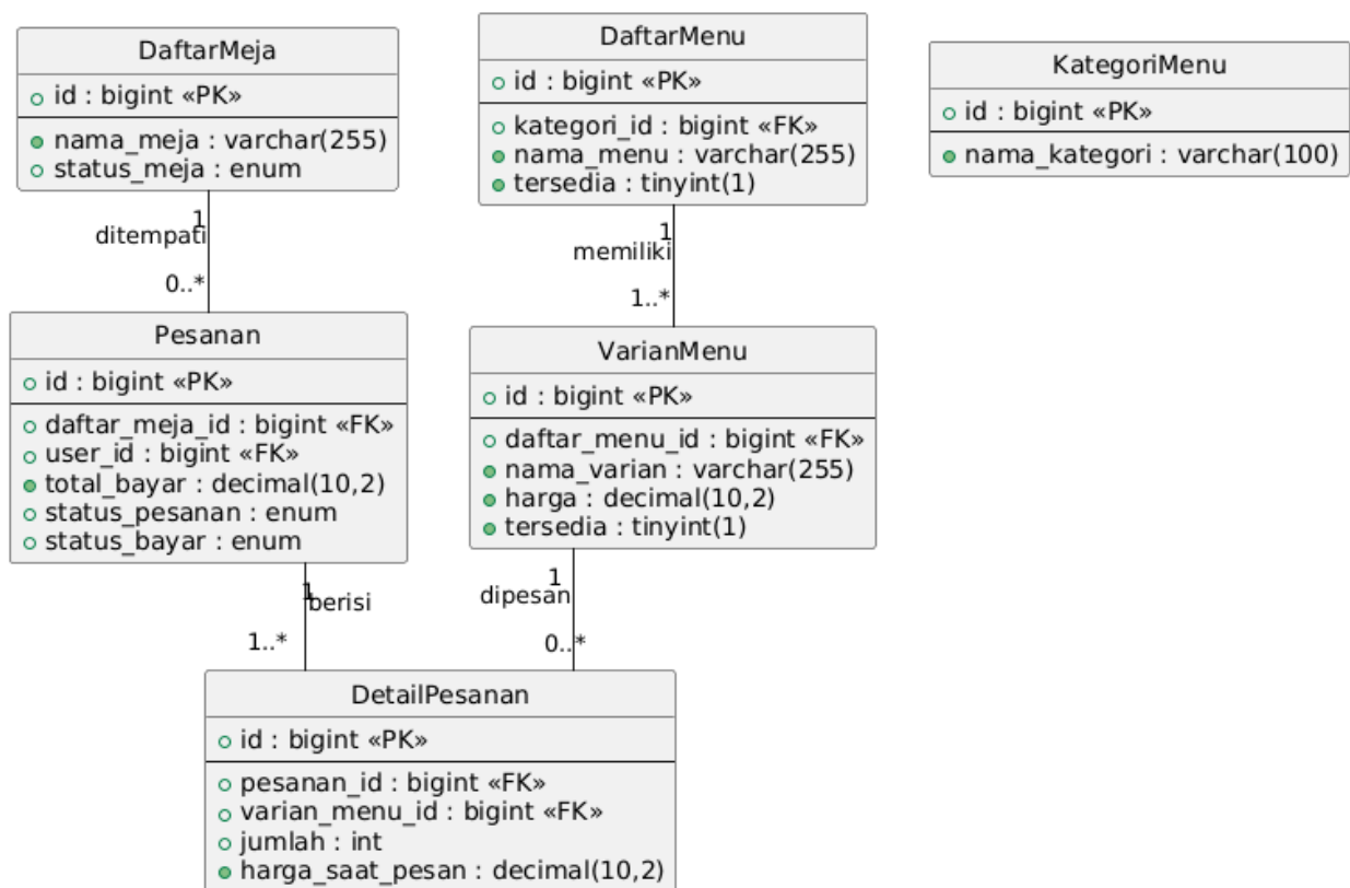
Gambar 4. 2 Class Diagram
