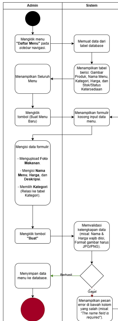
Gambar 4. 8 Activity Diagram Daftar Menu
