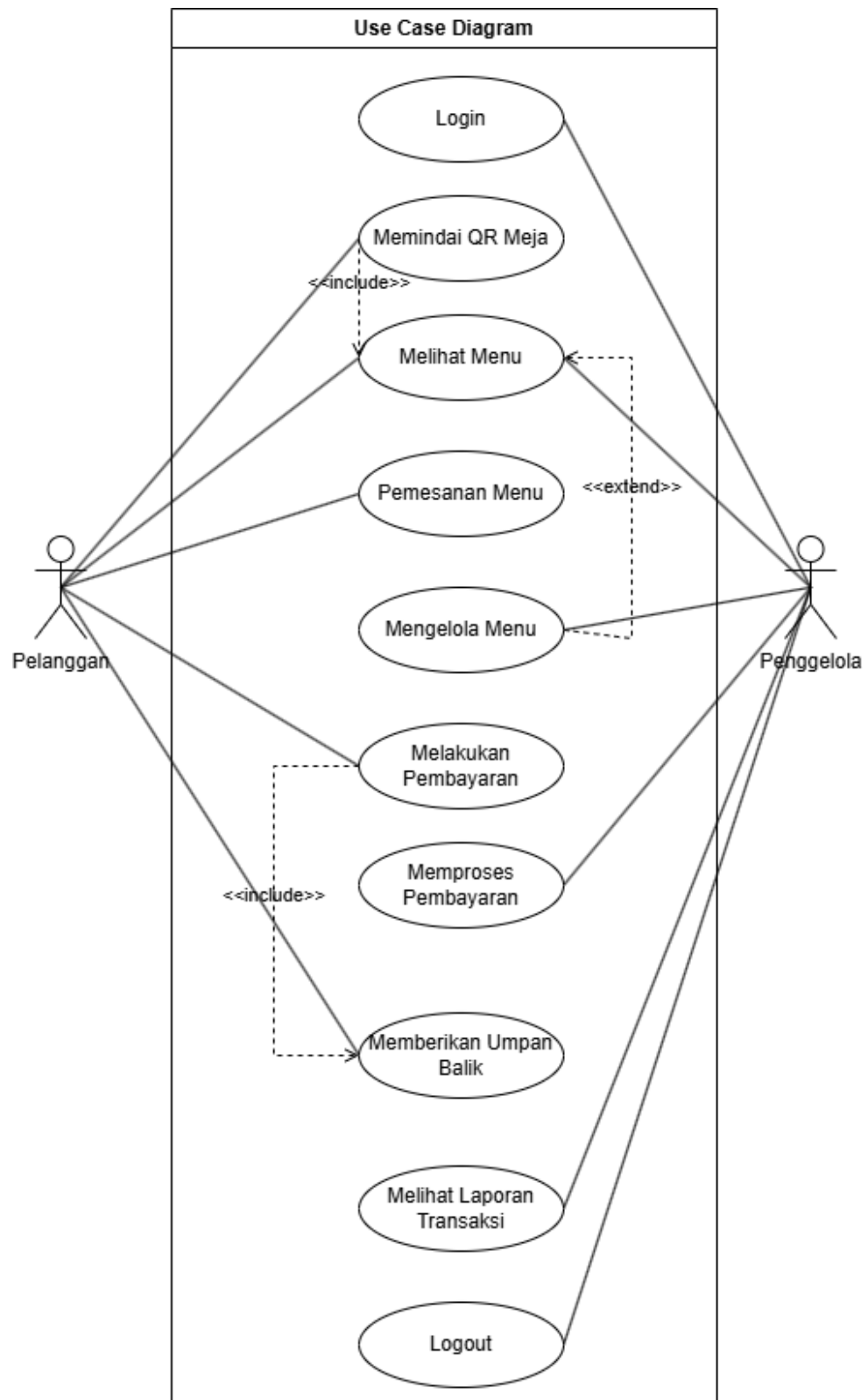
Gambar 3. 4 Simple Use Case Diagram
