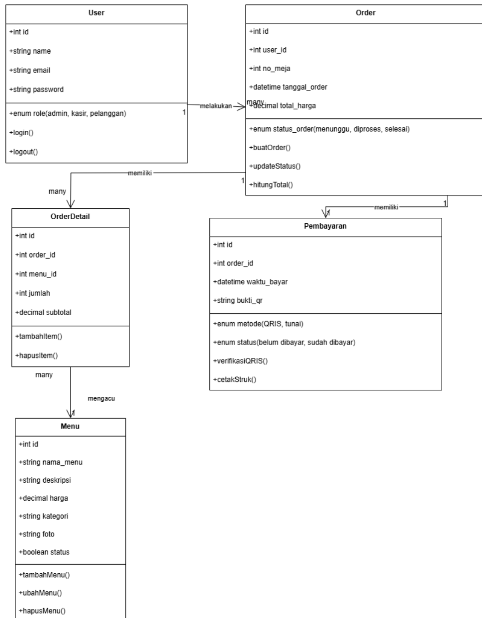
Gambar 3.5 Class Diagram
