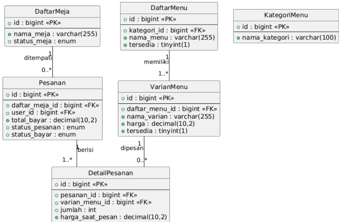
Gambar 4.2 Class Diagram
