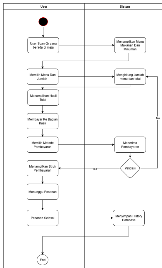
Gambar 3. 6 Activity Diagram
