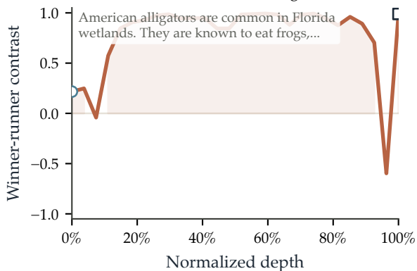
Qwen 2.5 7B on ARC-Challenge
