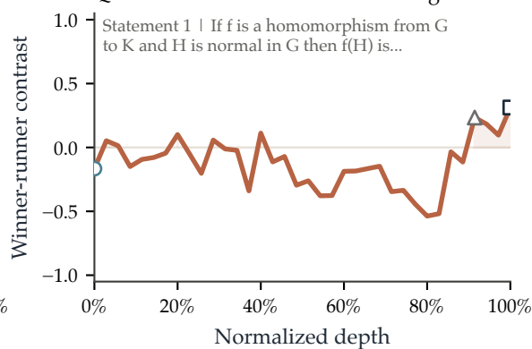
Qwen 2.5 3B on MMLU Abstract Algebra
