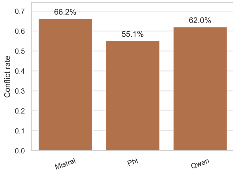
Items with wrapper conflict
