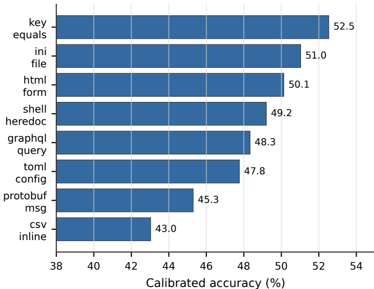
Accuracy by interface wrapper
