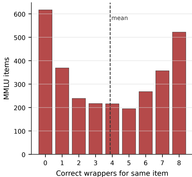
Item-level instability
