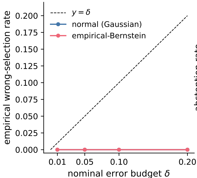
Observed ranking errors
