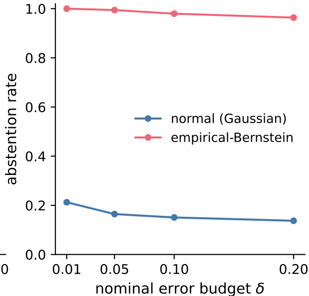
Strict selection: abstention
