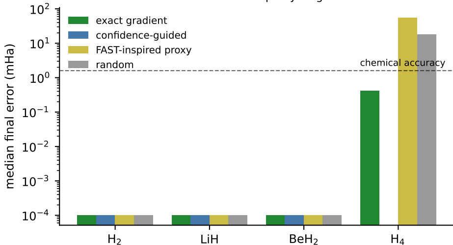
Molecular selection: proxy vs gradient
