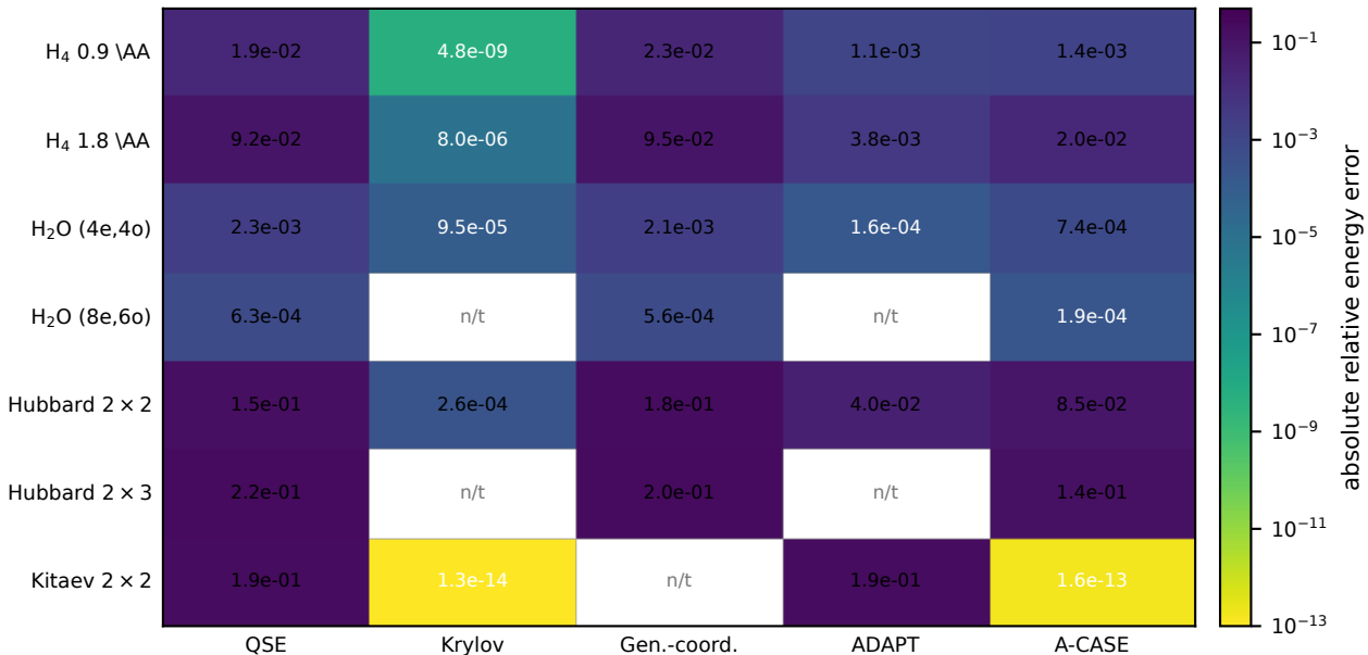
Matched-budget validation ladder (default A-CASE uses M = 9 )
