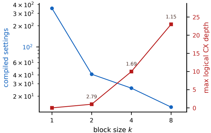
BeH 2 : trade does not pay
