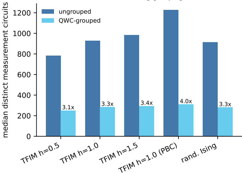
Qubit-wise-commuting grouping (n=4)
