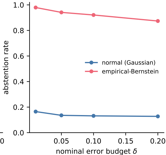
Cost of certification: abstention
