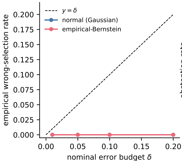
Certification holds: wrong \leq \delta
