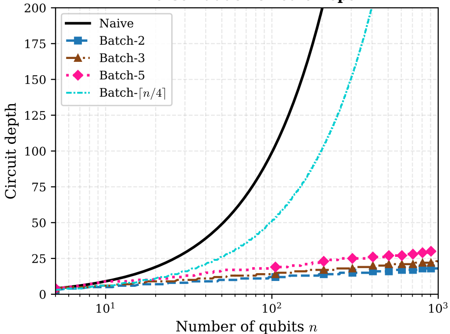
Inverse Ladder Circuit Depth
