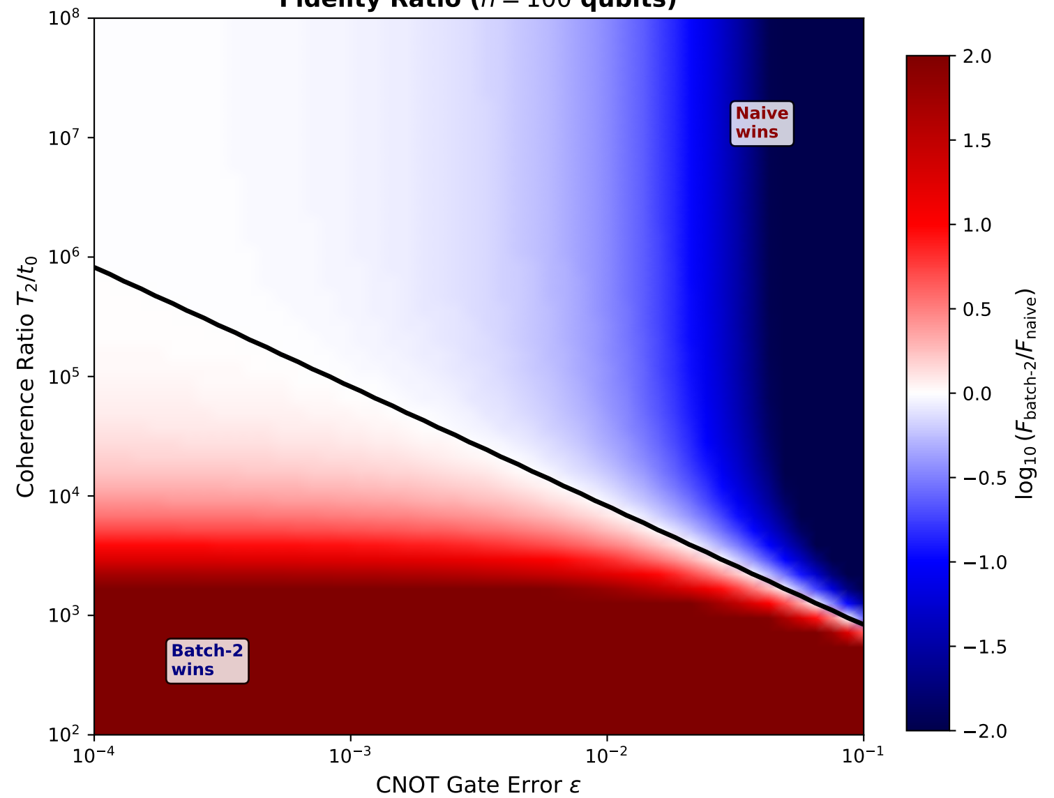
Fidelity Ratio ( n = 100 qubits)
