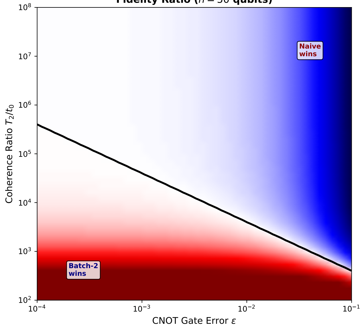
Fidelity Ratio ( n = 50 qubits)
