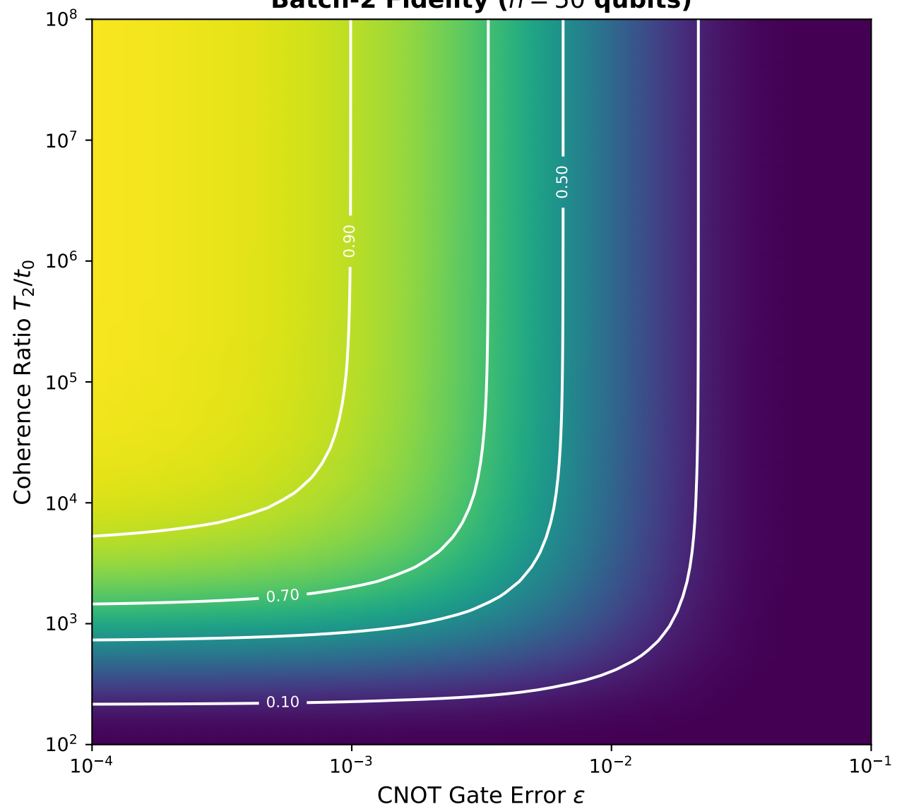
Batch-2 Fidelity ( n = 50 qubits)
