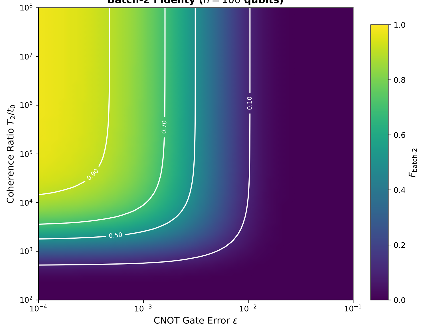
Batch-2 Fidelity ( n = 100 qubits)
