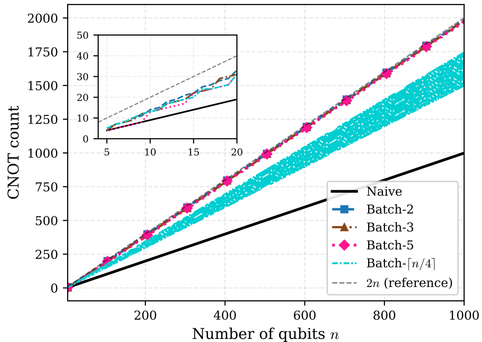
Inverse Ladder CNOT Count
