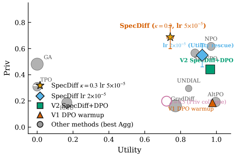
(b) Privacy-utility Pareto (area \propto Mem)
