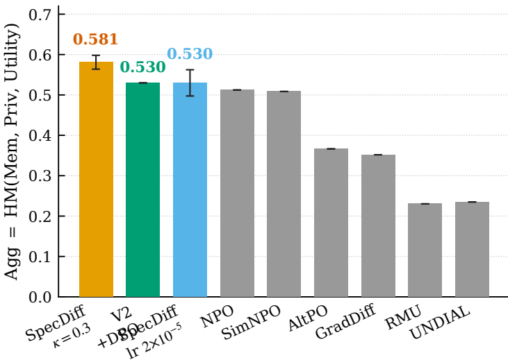
(a) Aggregate score (higher is better)
