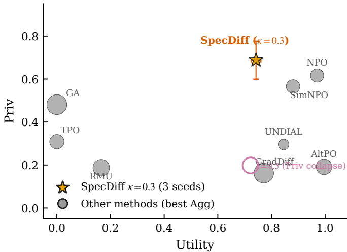
(b) Privacy-utility Pareto (area \propto Mem)
