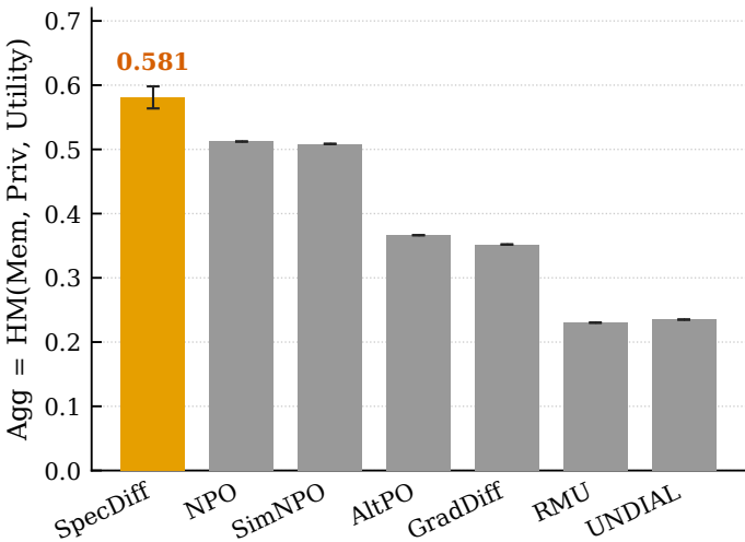
(a) Aggregate score (higher is better)
